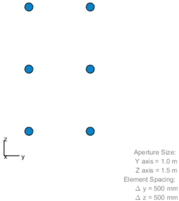
Array Geometry
